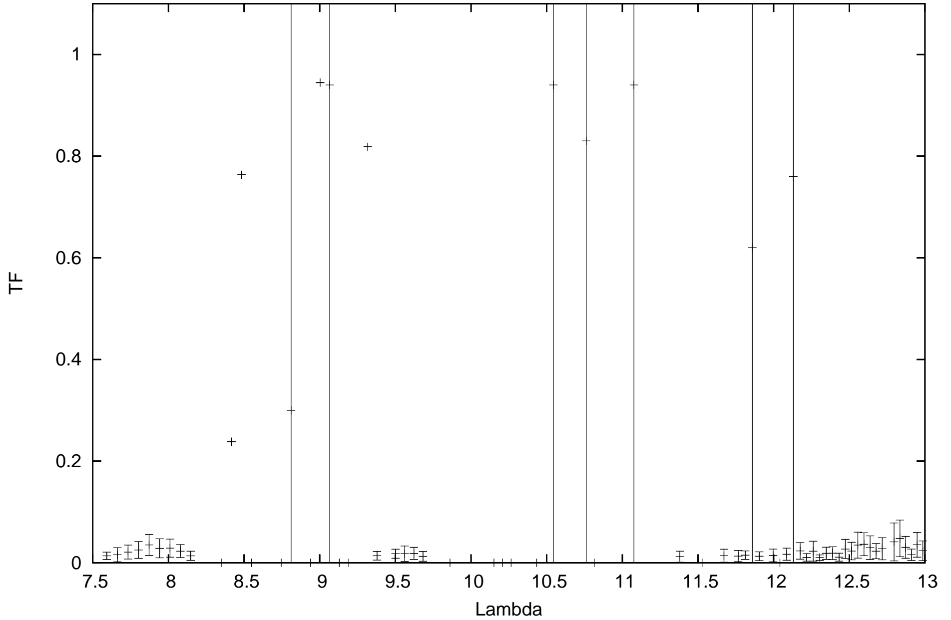
calHD018884_flux-1.93_diam12.27_r.MIDI.2009-01-04T01_12_30.000_HIGHSENS
