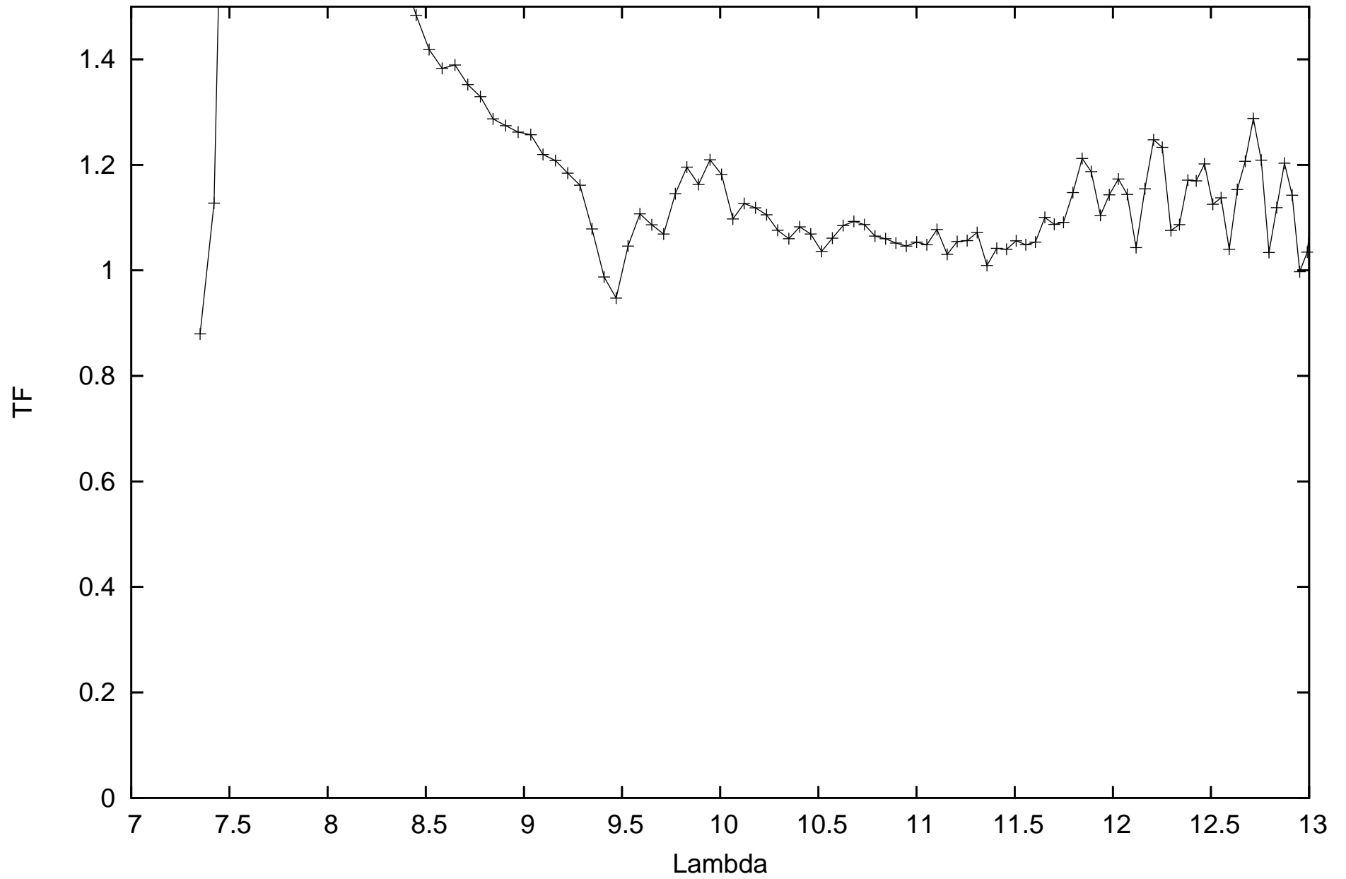
calHD081797_flux-1.49_diam9.14_r.MIDI.2008-12-27T07_59_20.180 SCIPHOT
