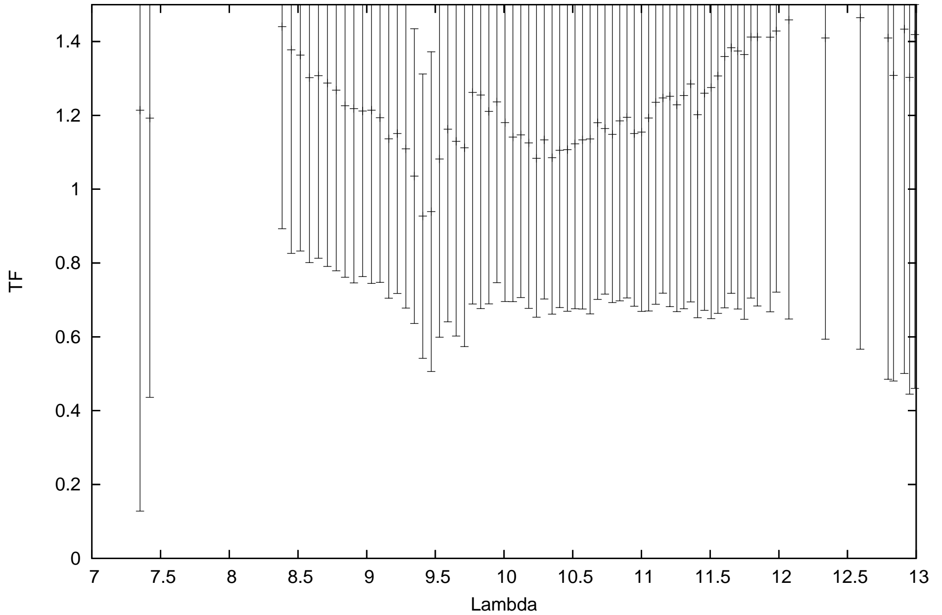
calHD048915_flux-1.39_diam6.09_r.MIDI.2008-12-25T08_37_04.015 SCIPHOT
