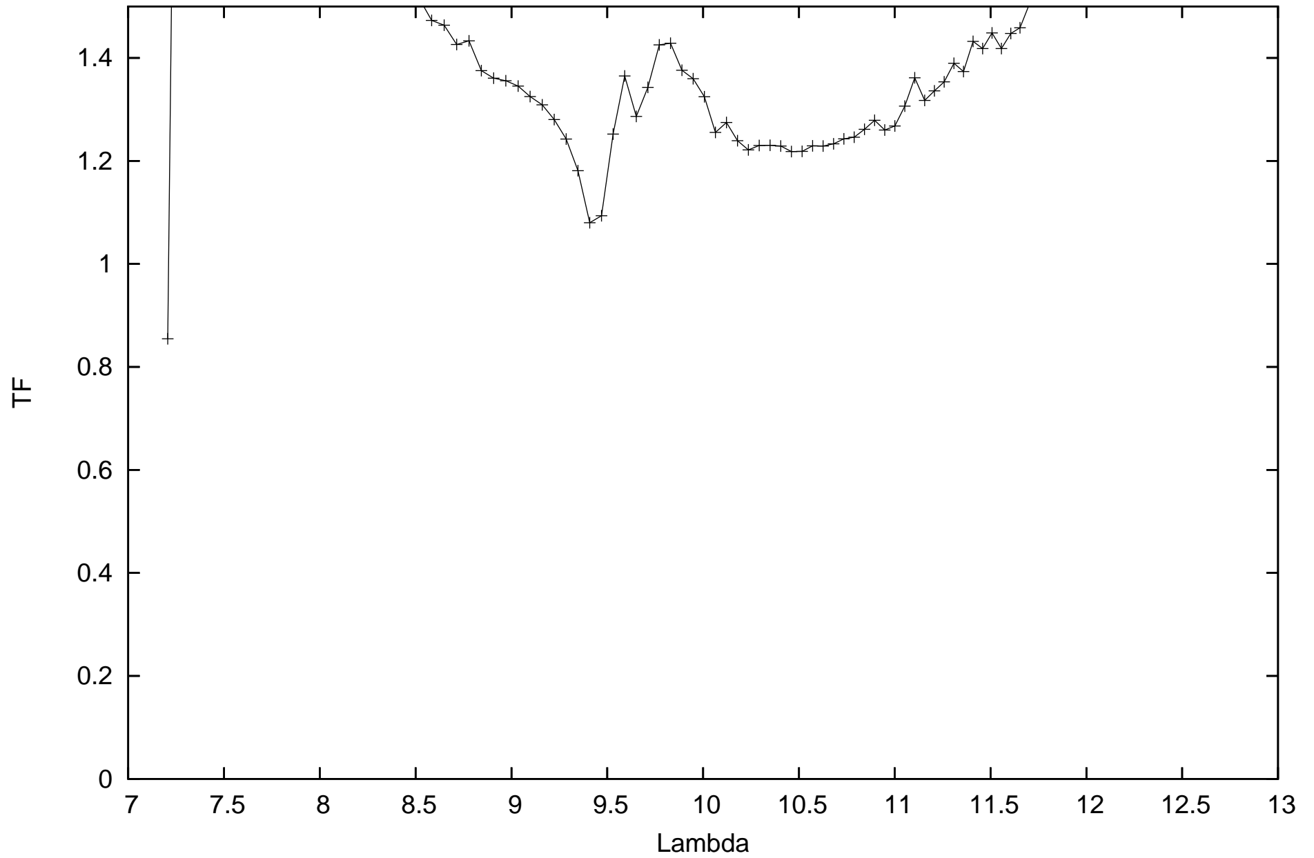
calHD048915_flux-1.39_diam6.09_r.MIDI.2008-12-25T05_43_40.179 SCIPHOT
