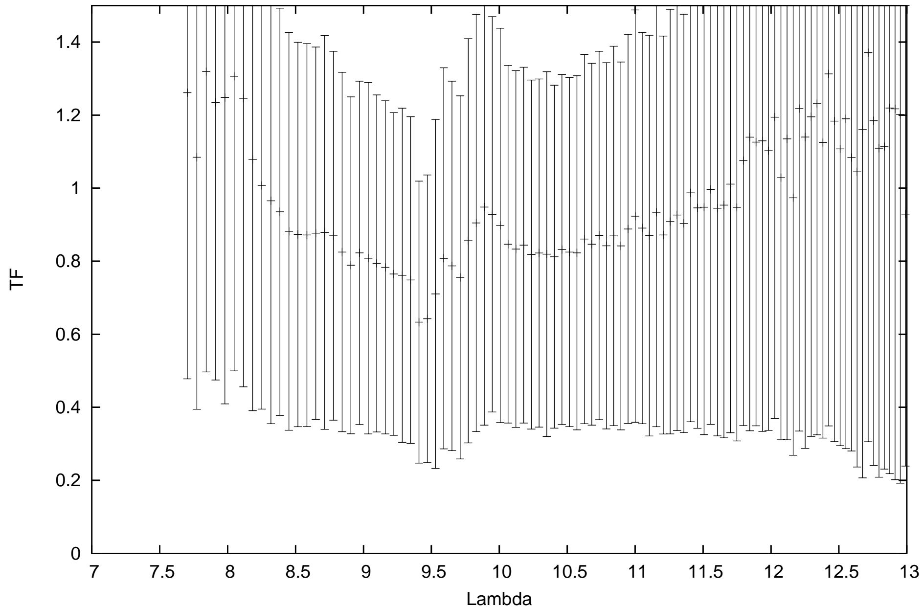
calHD049161_flux1.49_diam2.44_r.MIDI.2008-12-17T06_45_01.179 SCIPHOT
