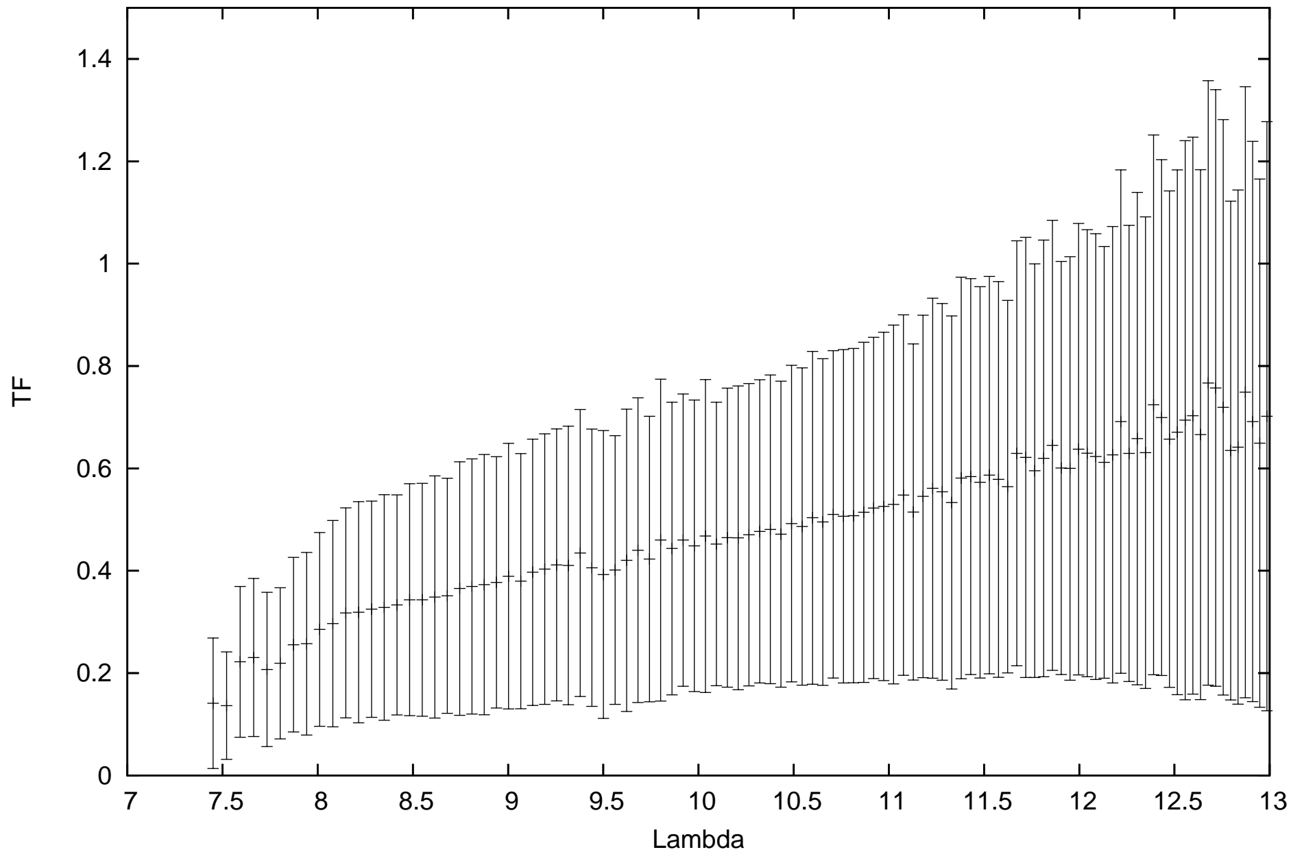
calHD025604_flux1.86_diam1.9_r.MIDI.2008-12-17T04_47_54.000_HIGHSENS
