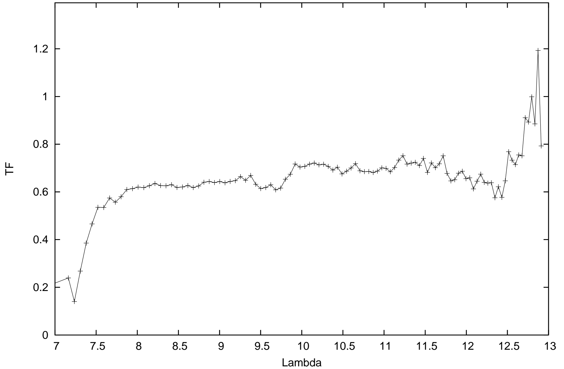
calHD004128_flux-0.44_diam5.23_r.MIDI.2008-12-06T00_43_23.000_HIGHSENS
