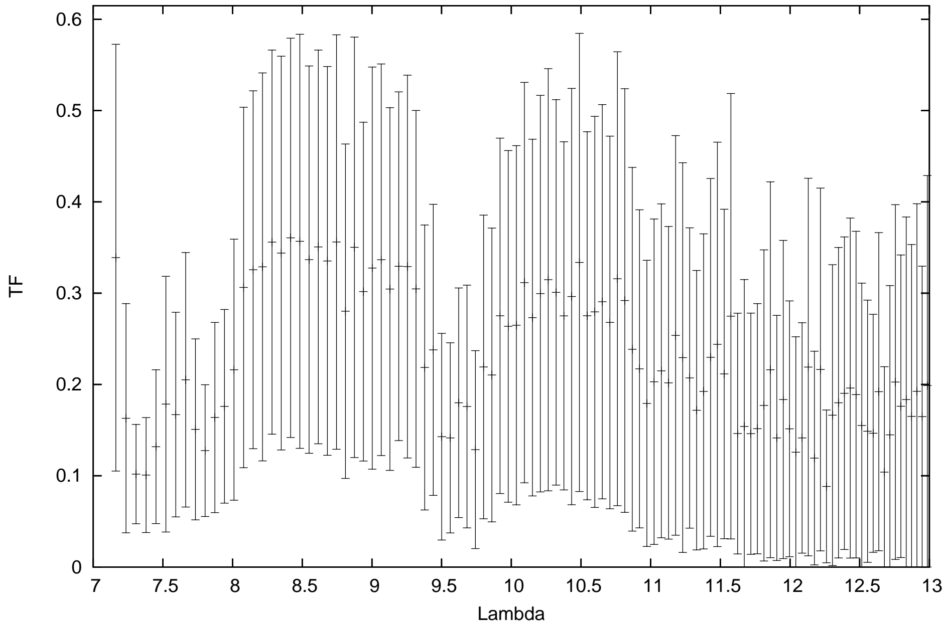
calHD216032_flux0.05_diam4.95_r.MIDI.2008-11-07T01_23_22.000_HIGHSENS
