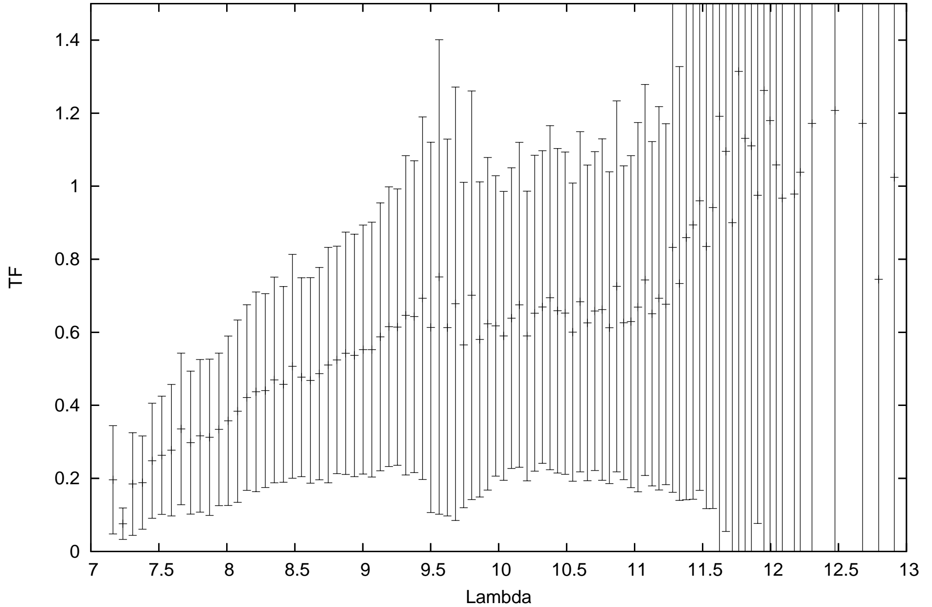
calHD224935_flux-0.85_diam7.24_r.MIDI.2008-10-27T03_30_36.000_HIGHSENS
