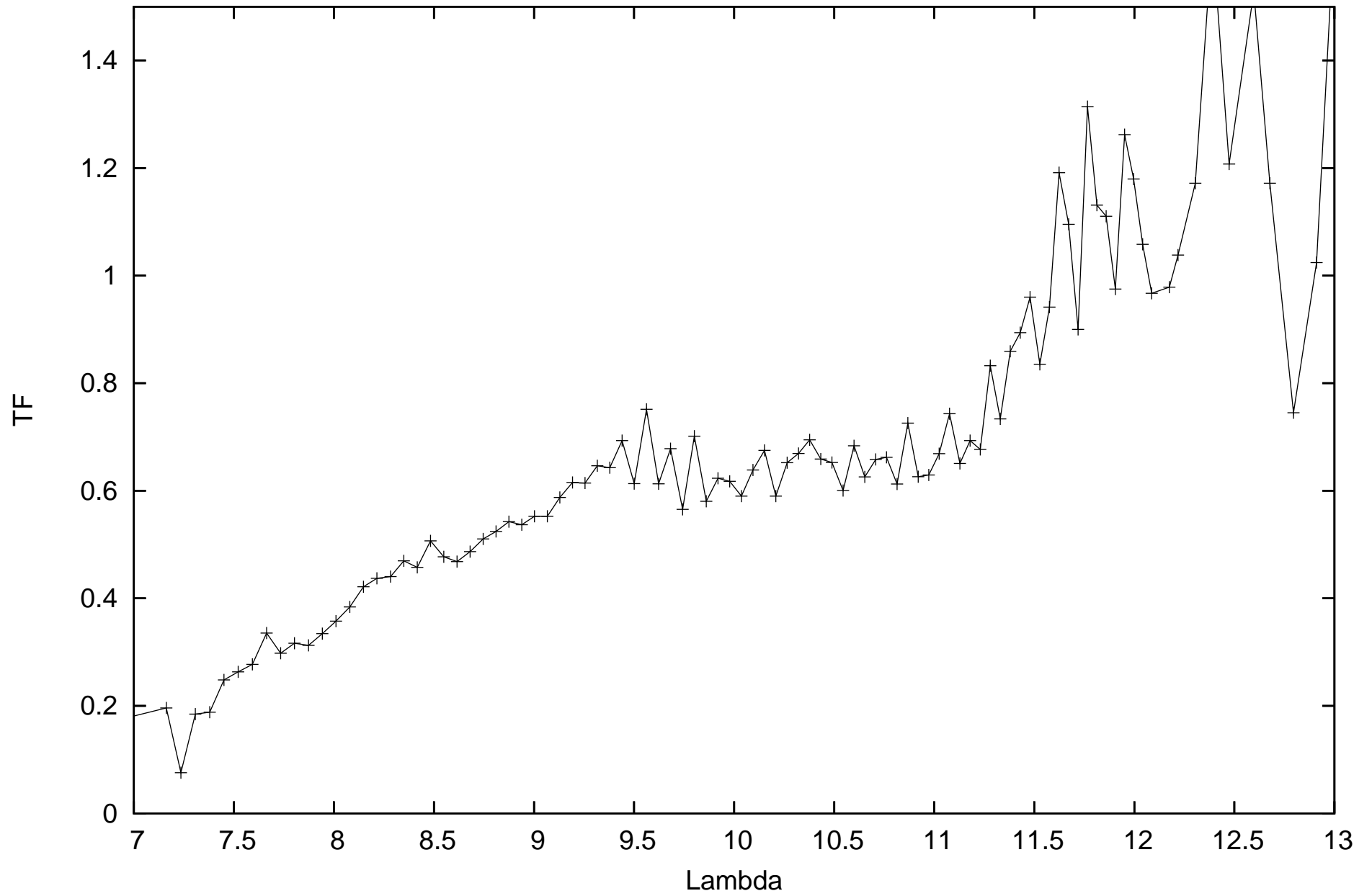
calHD224935_flux-0.85_diam7.24_r.MIDI.2008-10-27T03_30_36.000_HIGHSENS
