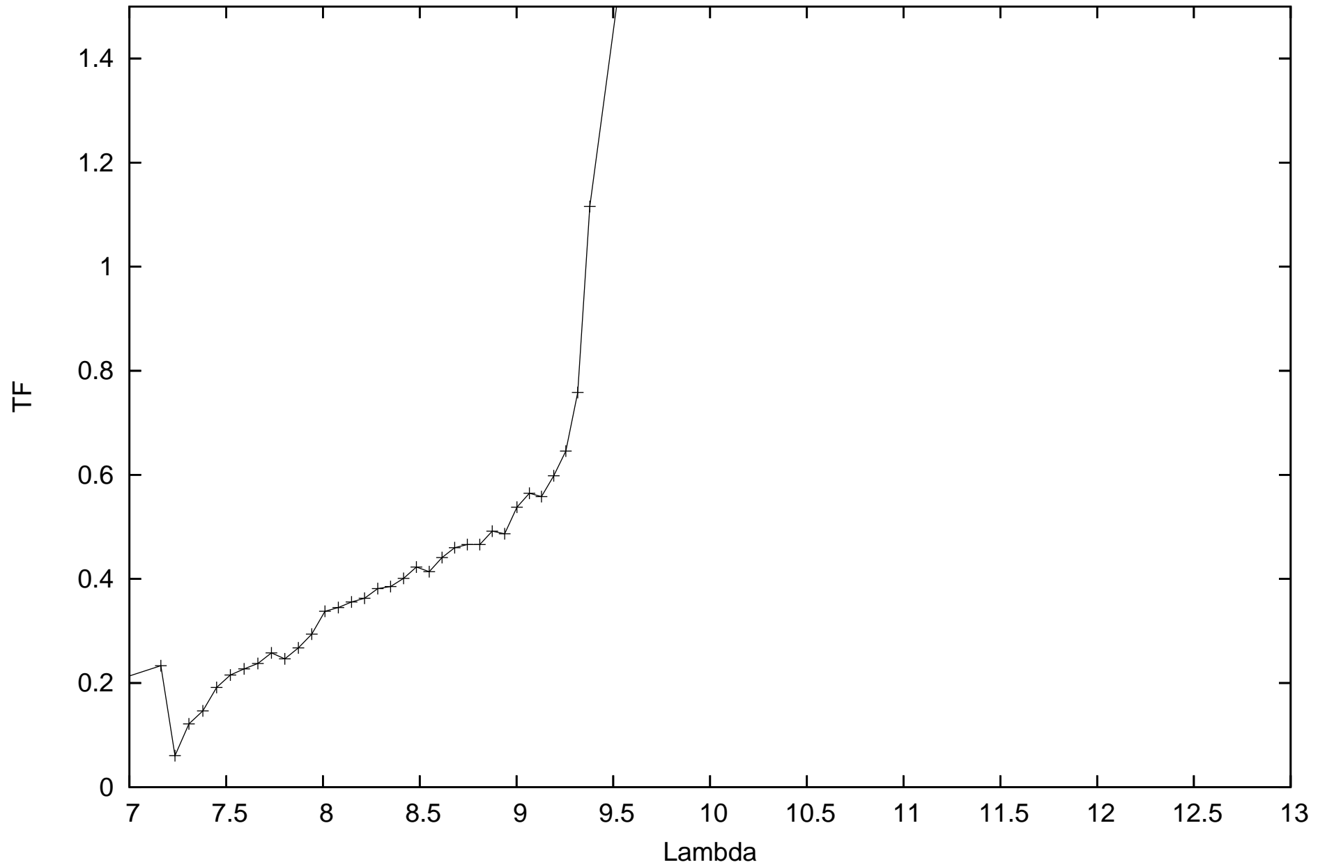
calHD189577_flux-0.25_diam5.44_r.MIDI.2008-10-09T23_52_32.000_HIGHSENS
