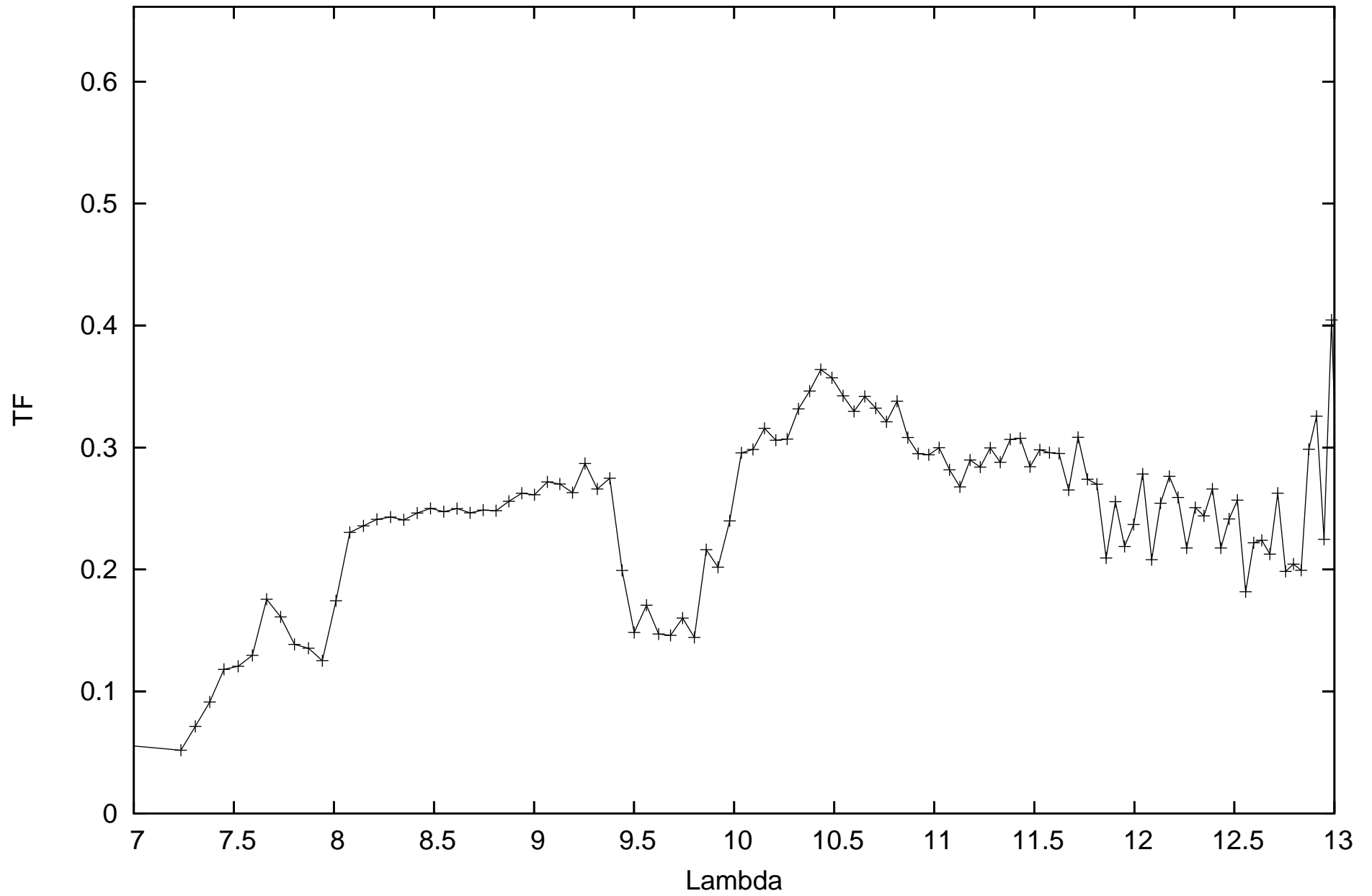
calHD004128_flux-0.44_diam5.23_r.MIDI.2008-10-04T07_51_55.000_HIGHSENS
