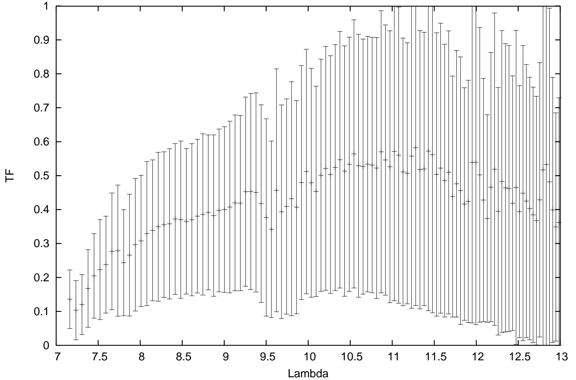
calHD004128_flux-0.44_diam5.23_r.MIDI.2008-10-04T06_01_15.000_HIGHSENS
