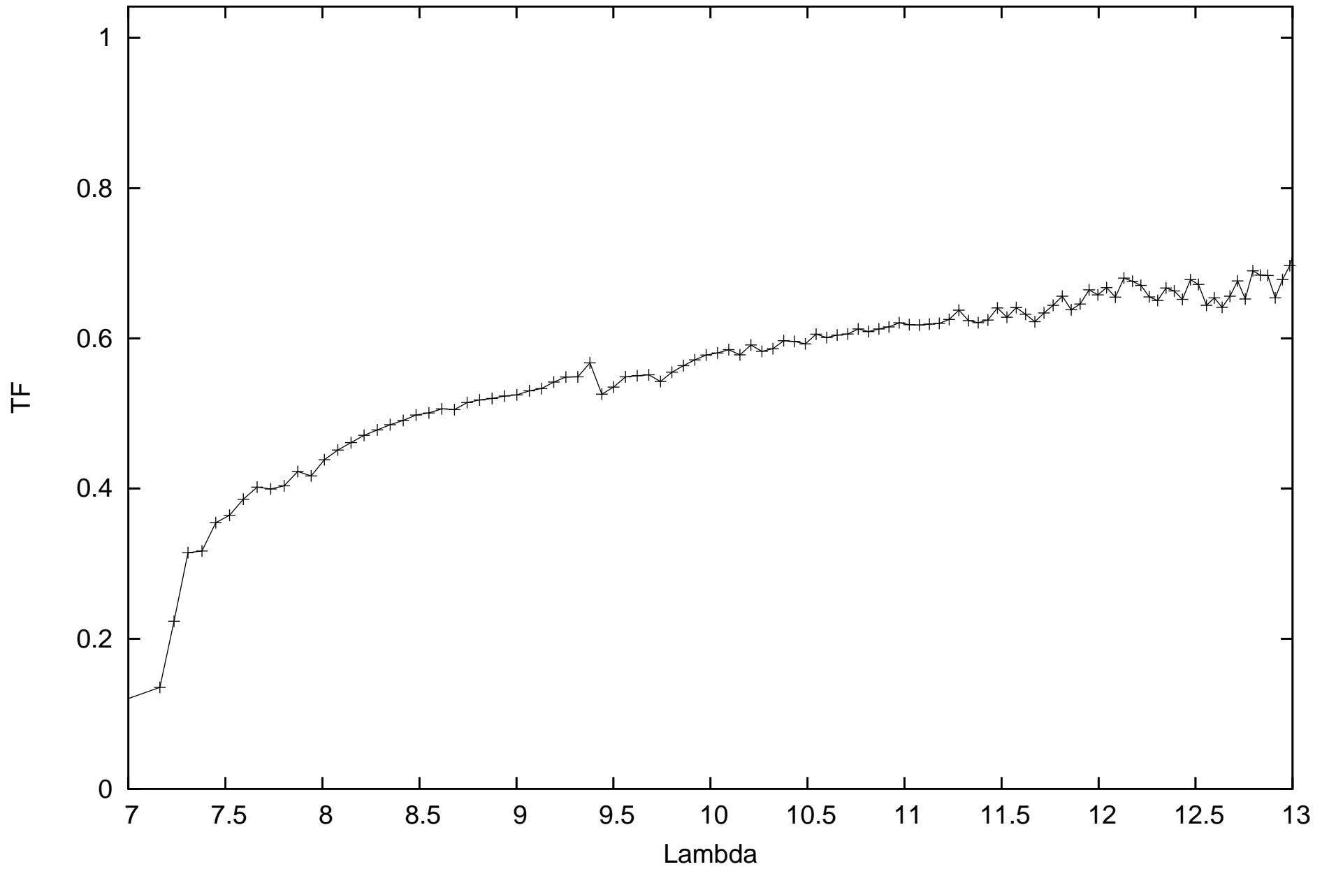
calHD167618_flux-1.82_diam11.66_r.MIDI.2008-09-24T00_56_09.000_HIGHSENS
