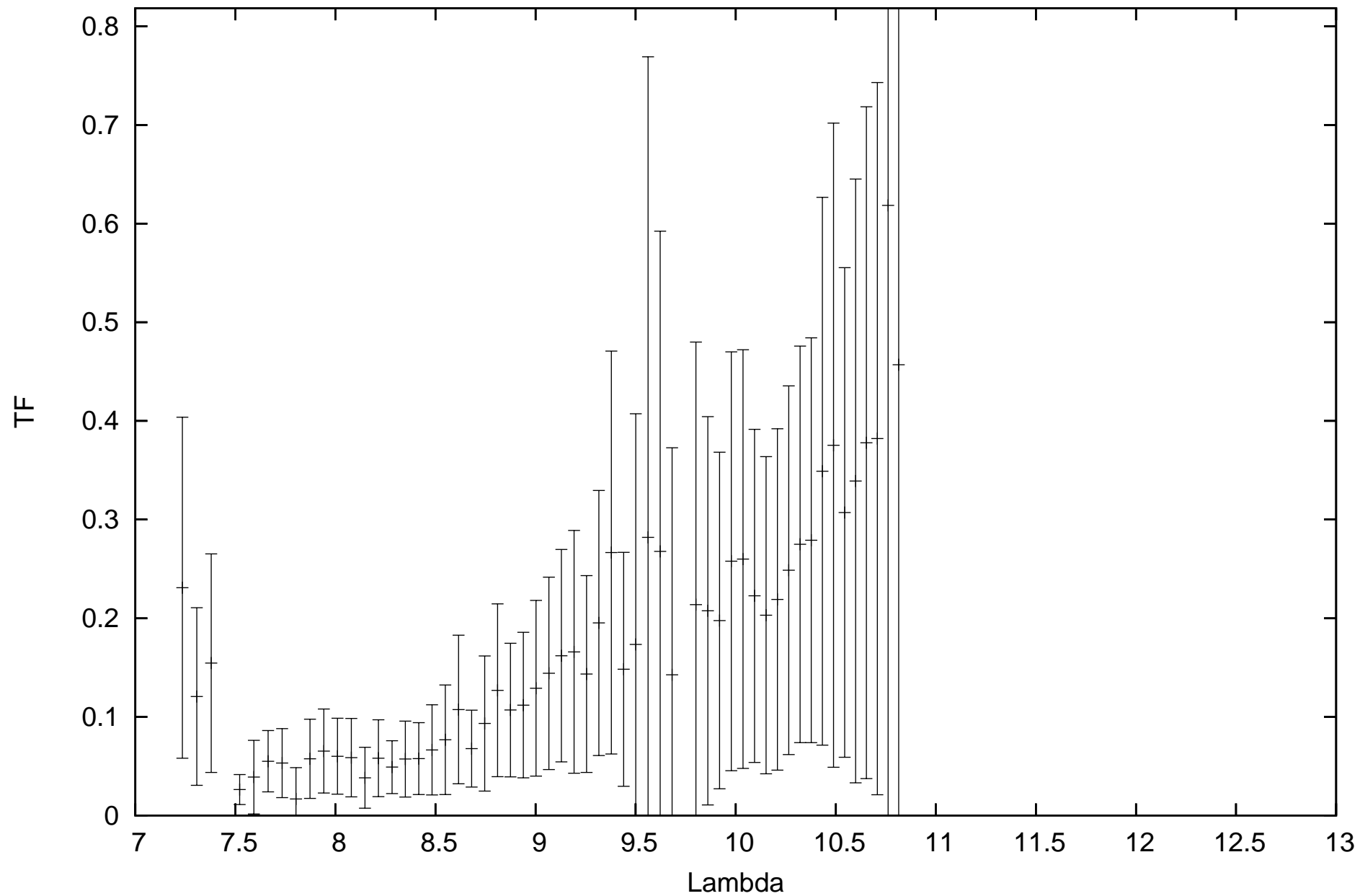
calHD001522_flux0.8_diam3.2_r.MIDI.2008-09-24T07_18_09.000_HIGHSENS
