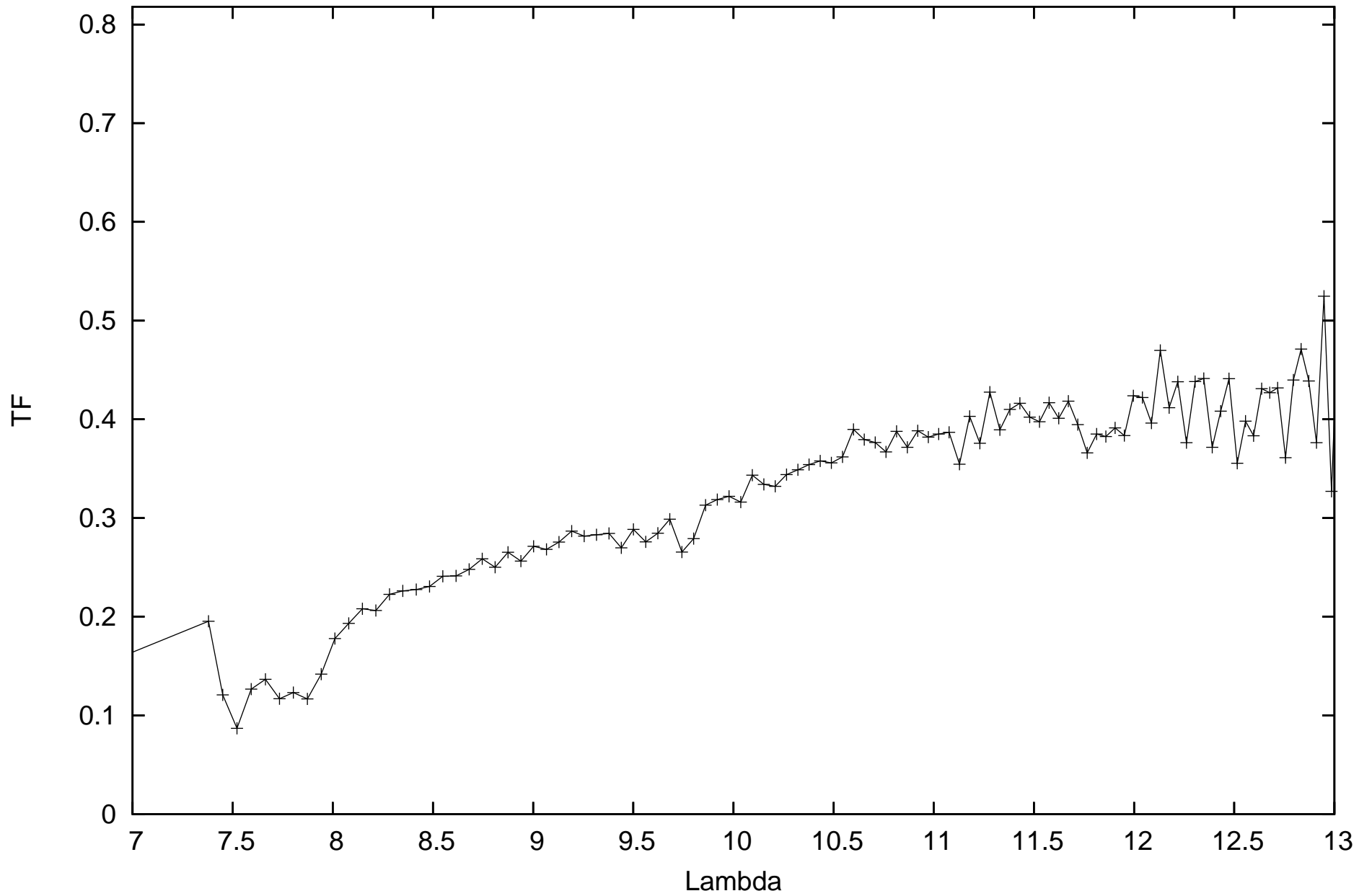
calhd101104_flux-9.9E+100_diam6.06_r.MIDI.2008-06-01T04_00_27.000_HIGHSENS
