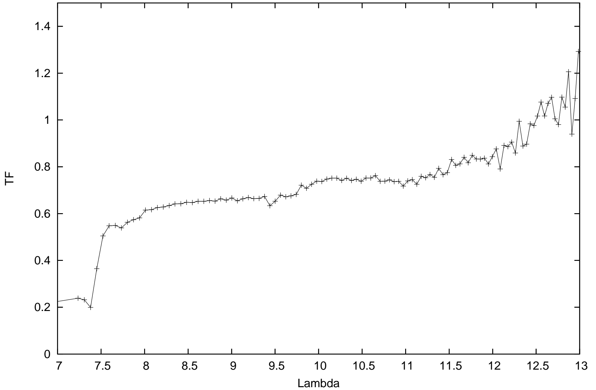
calhd101104_flux-9.9E+100_diam6.06_r.MIDI.2008-06-01T02_50_18.000_HIGHSENS
