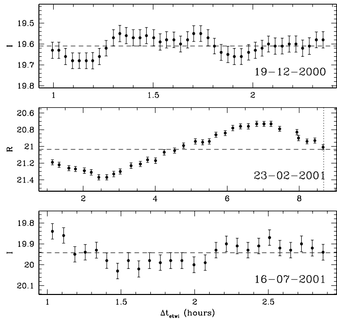
Fig. 11. Time sequences collected on 19-12-2000 ( I ), 23-02-2001 ( R ) and 16-07-2001 ( I ). The data have been corrected for airmass and differential zodiacal light contribution. The vertical dotted line is placed at the beginning of morning astronomical twilight.
