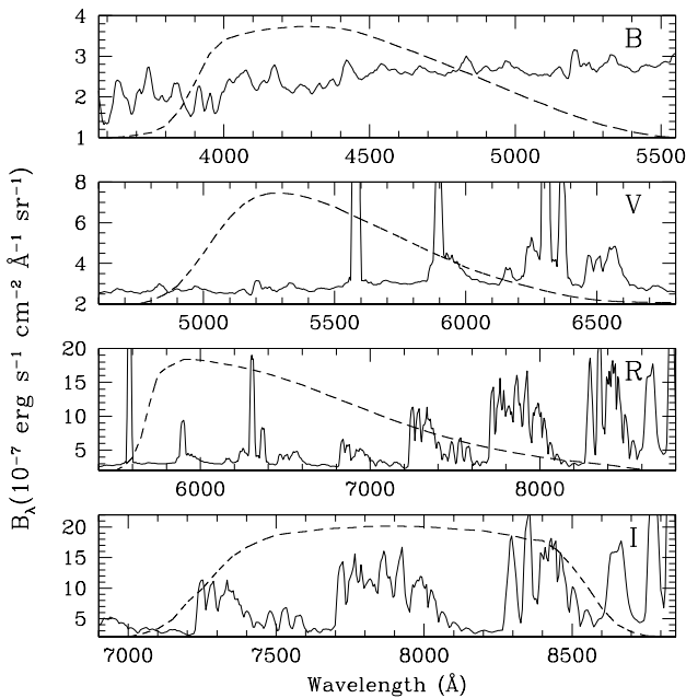
Fig. 1. Night sky spectrum obtained at Paranal on February 25, 2001 02:38UT in the spectral region covered by B , V , R and I passbands (from top to bottom). The original FORS1 1800 seconds frame was taken at 1.42 airmasses with a long slit of 1'' and grism 150I, which provide a resolution of about 22 Å (FWHM). The dashed lines indicate the passband response curves. Flux calibration was achieved using the spectrophotometric standard star Feige 56 (Hamuy et al. 1992) observed during the same night. The absence of an order sorting filter probably causes some second order overlap at wavelengths redder than 6600 Å.
