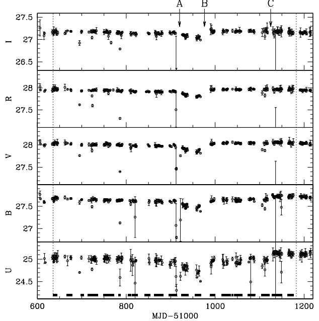
Fig. 2. UBVRI photometric zeropoints for FORS1 during the time range covered by sky brightness measurements presented in this work (vertical dotted lines). The thick segments plotted on the lower diagram indicate the presence of sky brightness data, while the arrows in the upper part of the figure correspond to some relevant events. A: water condensation on main mirror of UT1-Antu. B: UT1-Antu main mirror re-aluminisation after the water condensation event. C: FORS1 moved from UT1-Antu to UT3-Melipal. Plotted zeropoints have been corrected for extinction and colour terms using average values (see Appendix A).
