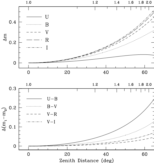
Fig. C.1. Upper panel: sky brightness variation (in \text{mag arcsec}^{-2} ) as a function of zenith distance expected from Eq. C.3 for f=0.6 . For each passband the mean Paranal extinction coefficients presented in Table A.1 were adopted. Lower panel: expected colour variation as a function of zenith distance. In both plots the upper scale reports the optical path-length X , expressed in airmasses.
