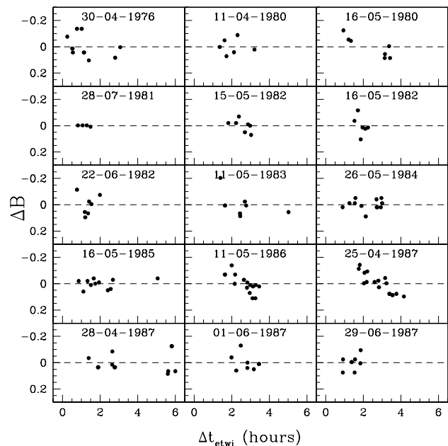
Fig. D.1. Zenith sky brightness at San Benito Mountain in the B passband from Walker (1988b). For clarity, the mean sky brightness has been subtracted to each time series.
