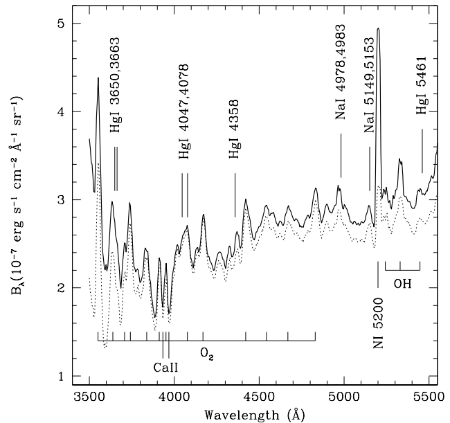
Fig. 16. Night sky spectrum obtained at Paranal on February 25, 2002 at 04:53 UT (see Figure 15). Marked are the expected positions for the most common lines produced by artificial scattered light (upper ticks) and natural atmospheric features (lower ticks). The dotted line traces part of the spectrum taken during the same night at 02:39 UT.
