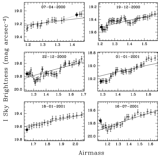
Fig. C.3. Sky brightness sequences on six different moonless nights at Paranal in the I passband, corrected for zodiacal light contribution. The dotted line connects chronologically the various data points, while the filled dot indicates the first observation in each time series. Finally, the solid line traces Eq. C.3 with f=0.7 .
