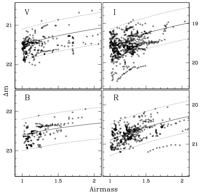
Fig. C.2. B, V, R and I sky brightness during dark time as a function of airmass. The solid line traces Eq. C.3, while the dotted lines are placed at \pm 0.4 \text{ mag} from this law.
