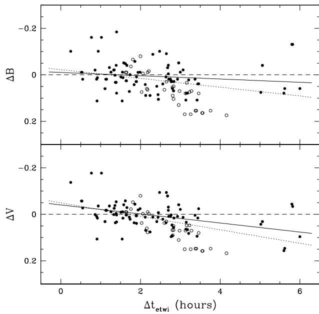
Fig. D.2. Variation in zenith sky brightness at San Benito Mountain with time after the end of astronomical twilight. Data have been corrected for differential zodiacal light contribution and all time series were normalised to the interpolated brightness at \Delta t_{etwi} = 2 hours. Dotted and solid lines trace a linear least squares fitting with and without the data of May 11, 1986 and April 25, 1987 respectively (empty circles). Data are from Walker (1988b).
