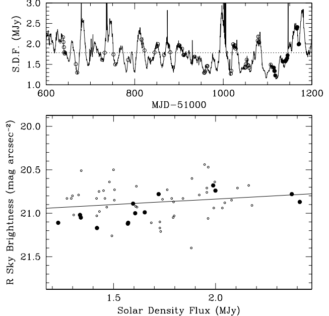
Fig. 13. Lower panel: nightly average sky brightness in the R passband vs. solar density flux. The filled circles represent data taken at \text{MJD} > 52114 , while the solid line indicates a linear least squares fit to all data. Upper panel: Penticton-Ottawa solar flux at 2800 MHz during the time interval discussed in this paper. The open circles indicate the values which correspond to the data presented in the lower panel and the dotted line is placed at the median value for the solar density flux.
