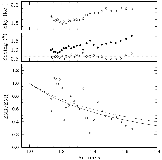
Fig. 17. Lower panel: peak signal-to-noise ratio measured for the same star on a sequence of 150 seconds I images obtained with FORS1 on July 16, 2001. Solid and dashed lines trace Eq. 3 for U and I passbands respectively. Middle panel: seeing measured by the Differential Image Motion Monitor (DIMM, Sandrock et al. 2000) at 5500 Å and reported to zenith (empty circles); each point represents the average of DIMM data over the exposure time of each image. The solid circles indicate the image quality (FWHM) directly measured on the images. Upper panel: sky background (in \text{ke}^- ) measured on each image.
