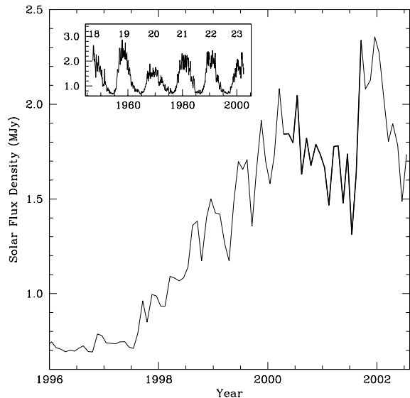
Fig. 6. Penticton-Ottawa Solar flux at 2800 MHz (monthly average). The time range covered by the data presented in this paper is indicated by the thick line. The upper left insert traces the solar flux during the last six cycles.
