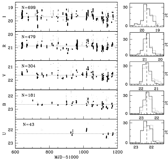
Fig. 7. Zenith corrected sky brightness measured at Paranal during dark time (thick dots) from April 1st, 2000 to September 30th, 2001. The selection criteria are: |b| > 10^\circ , |\lambda - \lambda_\odot| \geq 90^\circ , \Delta t_{twi} > 1 hour, FLI=0 or h_m \leq -18^\circ . Thin dots indicate all observations (corrected to zenith). The horizontal dotted lines are positioned at the average values of the selected points. The histograms trace the distribution of selected measurements (solid line) and all measurements (dotted line), while the vertical dashed lines are placed at the average sky brightness during dark time.
