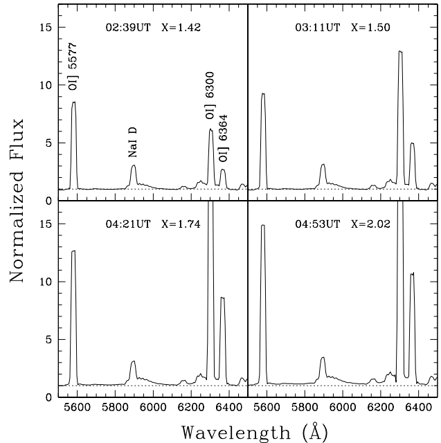
Fig. 15. Evolution of the night sky spectrum on February 25, 2001 in the wavelength range 5500-6500 Å. The original 1800 seconds spectra were obtained with FORS1, using the standard resolution collimator and a long slit 1'' wide (see also the caption of Figure 1). In each panel the starting UT time and airmass X are reported. For presentation the four spectra have been normalised to the continuum of the first one in the region 5600-5800 Å.
