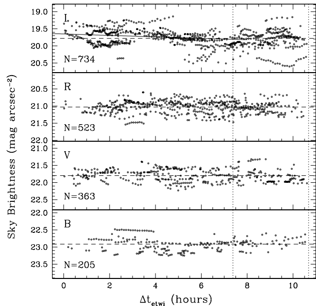
Fig. 9. Dark time Paranal night sky brightness, corrected for zodiacal light contribution, as a function of time distance from evening twilight. The vertical dotted lines indicate the shortest and longest night (7.4 and 10.7 hours respectively, astronomical twilight to twilight), while the dashed horizontal line is placed at the average value in each passband.
